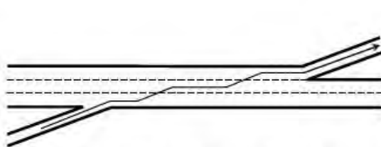
(a) Two-Sided Weaving Section with Single-Lane Ramps
